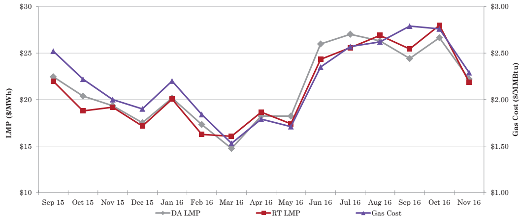
Figure 3-2 SPP Energy Prices and Gas Prices
