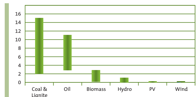
Figure 6. External Costs of electricity production in the EU in Eurocent/kWh. Source: Data from the European Commission-ENERGIE Programme (European Union 5th Research and Technological Development Framework Programme). G-8 RETF, 2001, Figure 4, p. 19.
